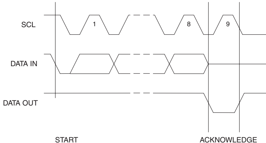
Figure 4-6. Output Acknowledge
