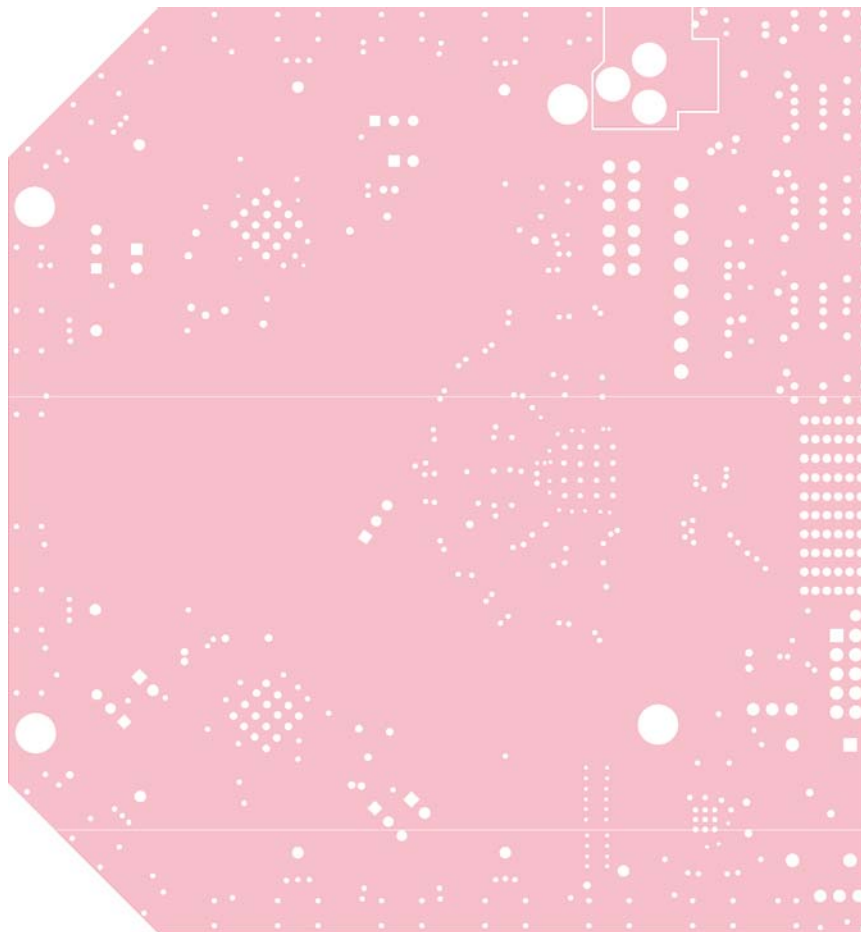
Figure 82. Evaluation Board Layout, Ground Plane
